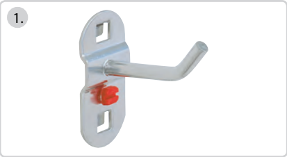
Tool holder with oblique hook • impact and scratch resistant • coating stamped base plate 1,5mm • „GS“ safety tested tool holder
